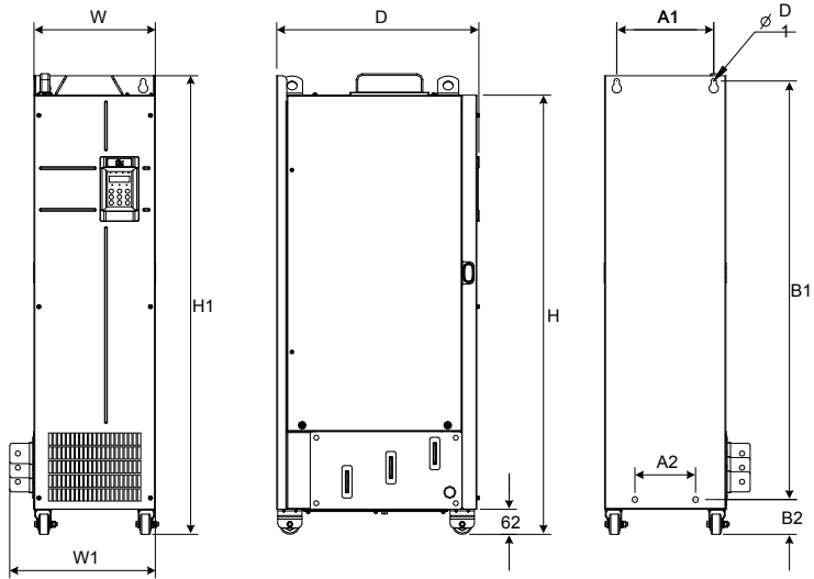
Figure 1-4 Overall dimensions of MD290T200G-L to MD290T450G-L and MD290T220P-L to MD290T500P-L (with output AC reactor)
