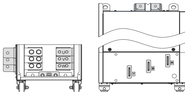
Figure 2-3 Main circuit terminals of MD290T200G to MD290T450G and MD290T220P to MD290T500P
