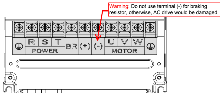
Figure 2-2 Main circuit terminals of MD290T45G/55P to MD290T160G/200P (sheet metal housing)
