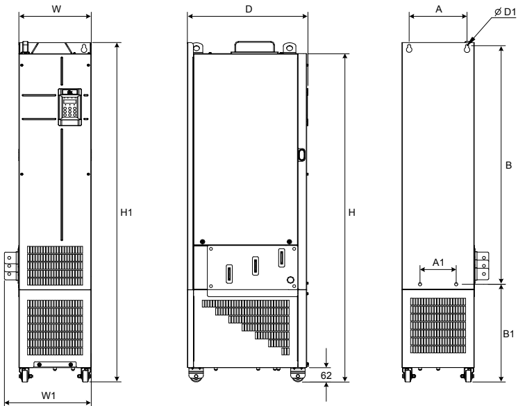
Figure 1-4 Overall dimensions of MD290T200G-L to MD290T450G-L and MD290T220P-L to MD290T500P-L (with output AC reactor)
